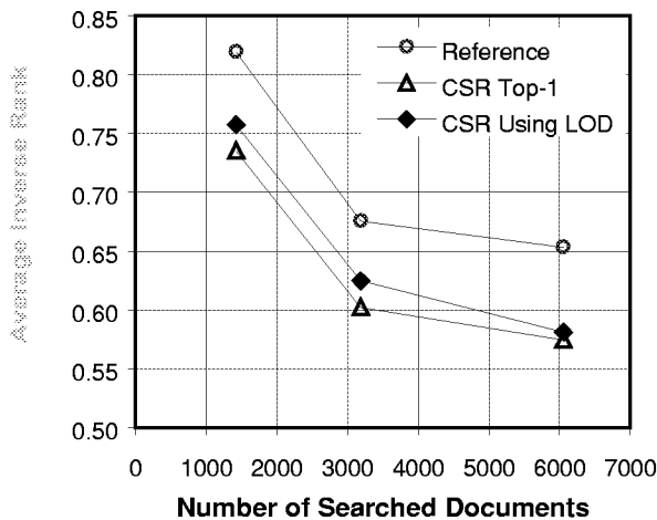
Figure 3: Chart of the data in Table 2. Each line shows the retrieval performance for a different source of text, under three different document sets.
