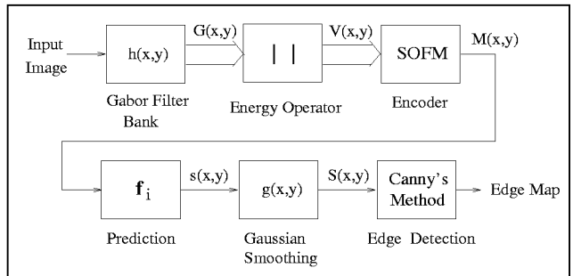
Figure 1: Texture Edge Detection System.
