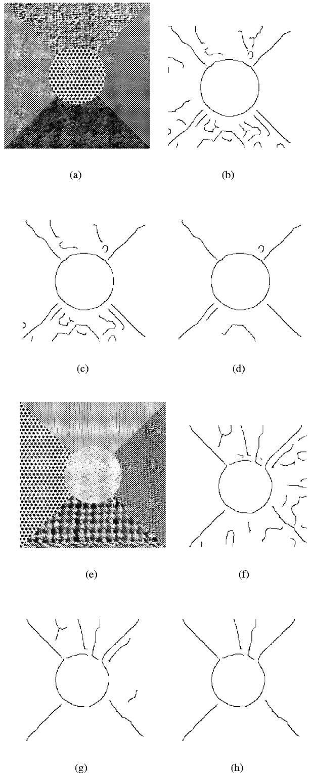
Figure 3: (a) Test image 1, and texture edge detection results by thresholding at (b) 0.7, (c) 0.75, (c) 0.8. (e) Test image 2, and results by thresholding at (f) 0.6, (g) 0.7, (h) 0.75.
