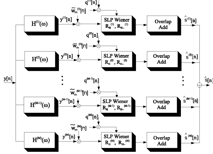
Figure 1: Overall enhancement system.
