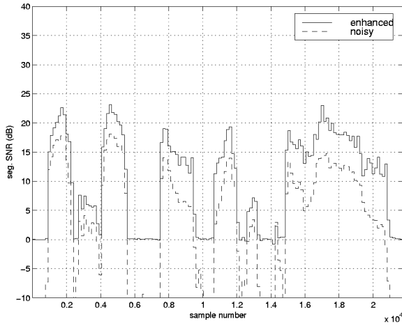
Figure 3: Segmental SNRs of enhanced and noisy (shown in Figure 2) versus sample number using Equation 5 with N_s = 150 .
