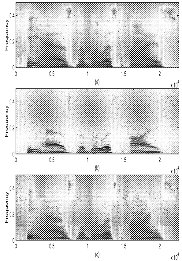
Figure 4: Spectrograms of (a) clean ("He has the bluest eyes"), (b) noisy and (c) enhanced.
