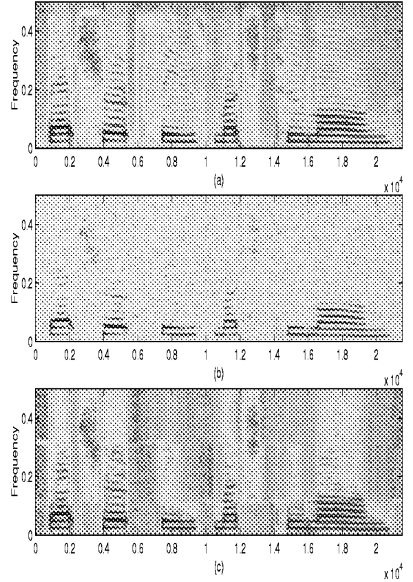
Figure 2: Spectrograms of (a) clean (“That shirt seems too long”) (b) noisy and (c) enhanced.
