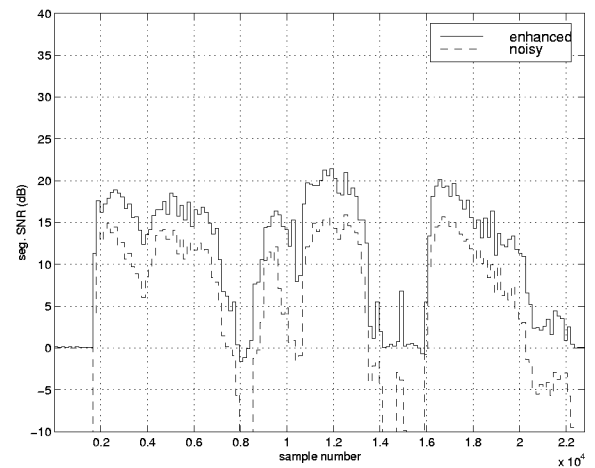
Figure 5: Segmental SNRs of enhanced and noisy (shown in Figure 4) versus sample number using Equation 5 with N_s = 150 .
