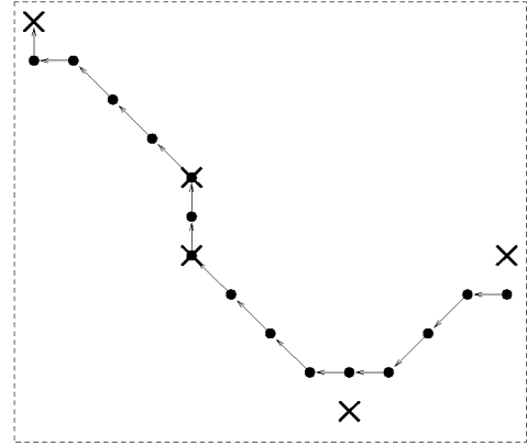
Figure 2: Control points (X marks) and boundary pixels (circles) in a temporal context window. Context: NW direction, run of 4.
