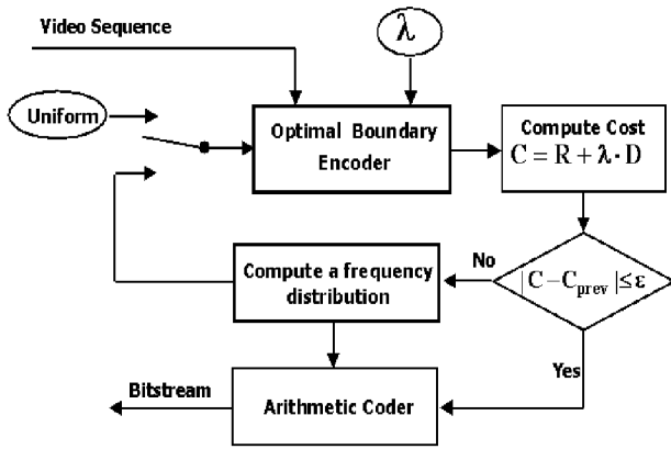
Figure 5: The entropy encoder structure.
