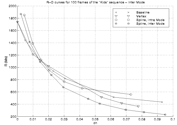
Figure 6: Rate-Distortion curves.
