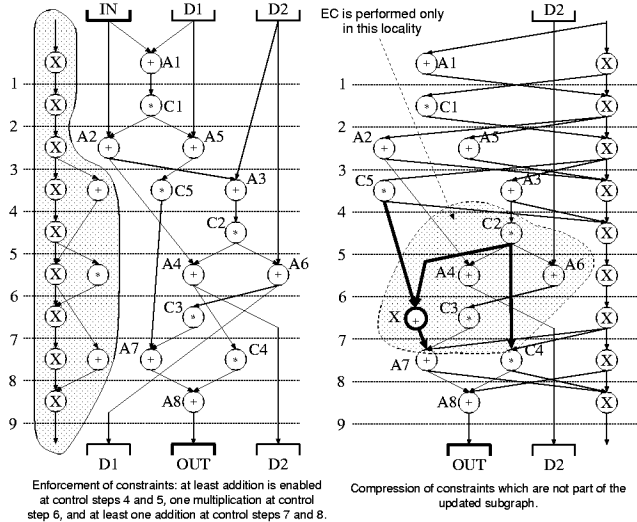
Figure 6: Constraint augmentation and subgraph compression for pre- and post-processing for EC of operation scheduling.
