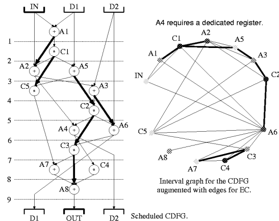
Figure 2: An example of addition of type-I constraints to the graph coloring problem for EC.
