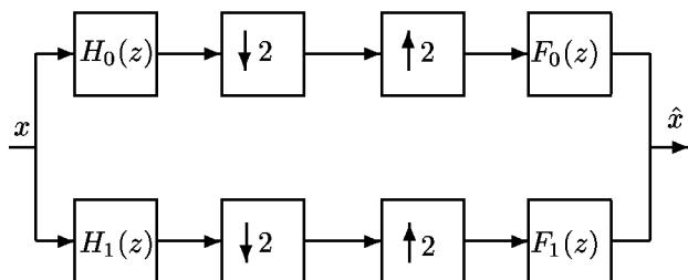
Figure 1: Two-channel filter bank
