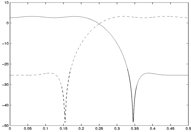
Figure 4: Frequency response of H^\infty optimal synthesis filters
