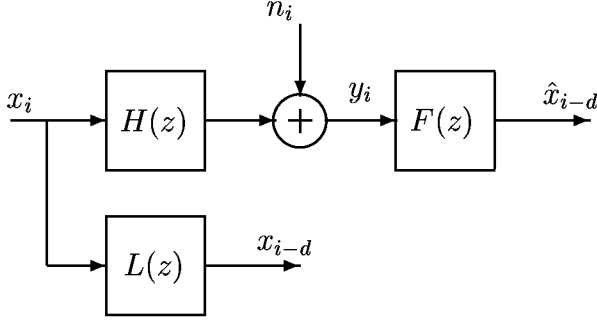
Figure 2: Polyphase equivalent to 2-band noisy filter bank
