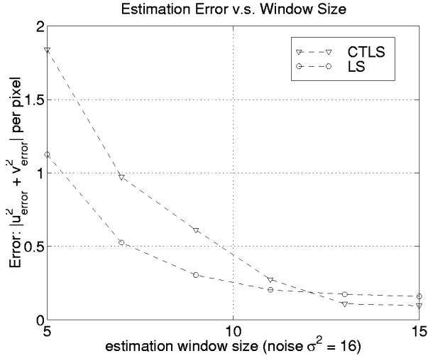
Figure 4: Estimation error as a function of window size
