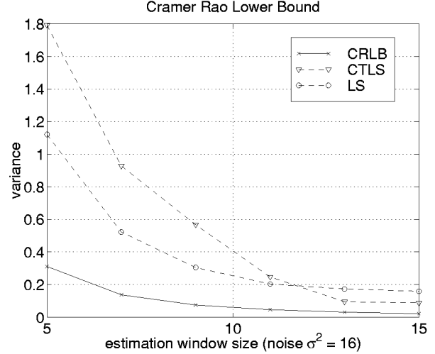
Figure 3: Variance of estimates as a function of window size
