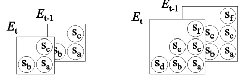
Figure 1: Left: the neighborhood structure for derivative estimation. Right: pixels used for optical flow estimation at position s_a .
