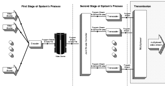
Figure 1: Block diagram of the two-stage joint bit-rate coding system.
