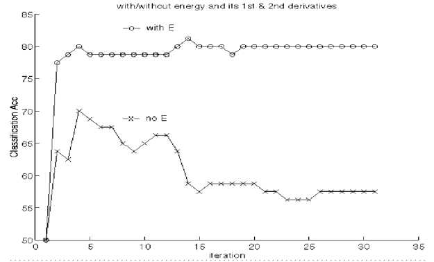
Figure 2: accent classification accuracy with/without energy feature
