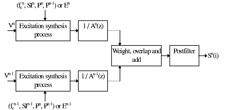
Figure 2 MPS-PIC decoding process
