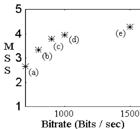
Figure 4 Mean Subjective Scores (MSS) for the test schemes at (a) 700 BPS (b) 800 BPS (c) 900 BPS (d) 1.0kbps and (e) 1.5kbps
