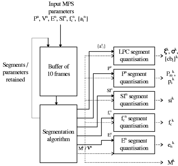
Figure 3 Segmental Quantisation model
