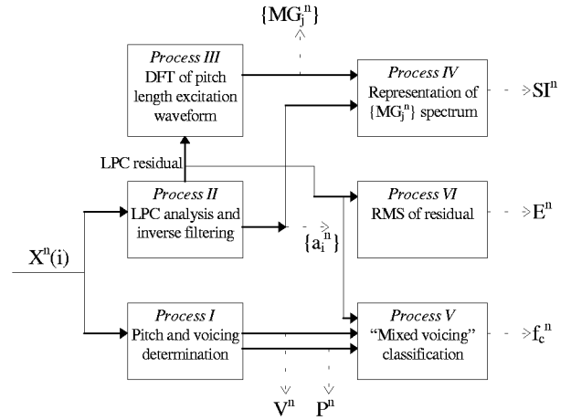
Figure 1 MPS-PIC encoding process
