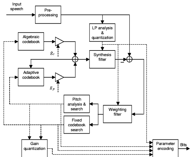
Figure 1. Principle of CELP encoder with LPAS.
