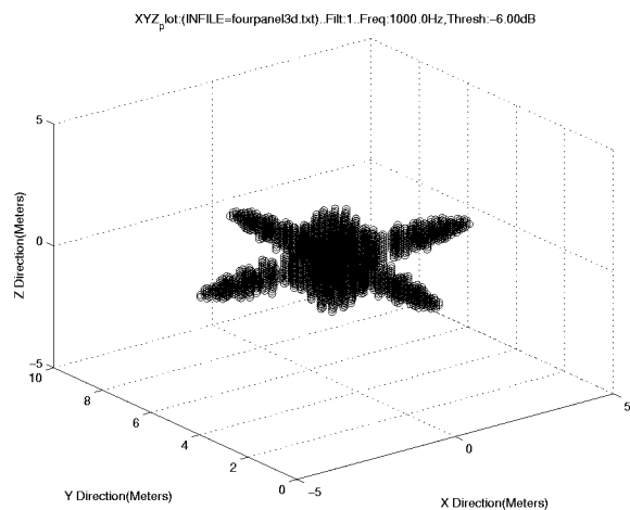
Figure 7: Locus of Points with Response Greater than -6dB at F=1kHz for Array II
