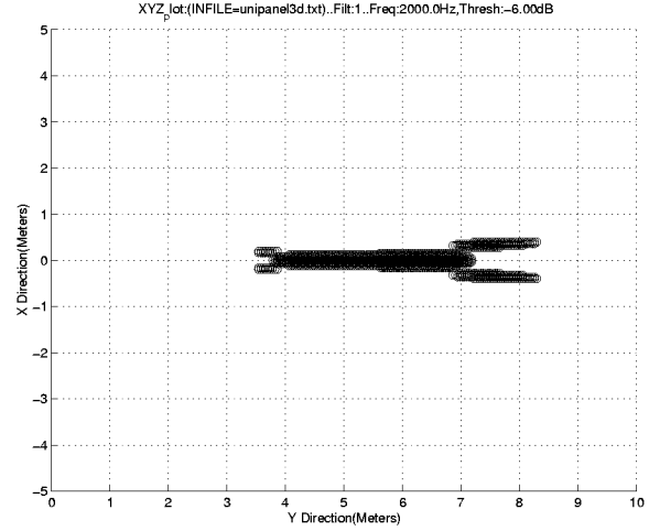
Figure 4: X-Y View of Points with Response Greater than -6dB at F=2kHz for Array I
