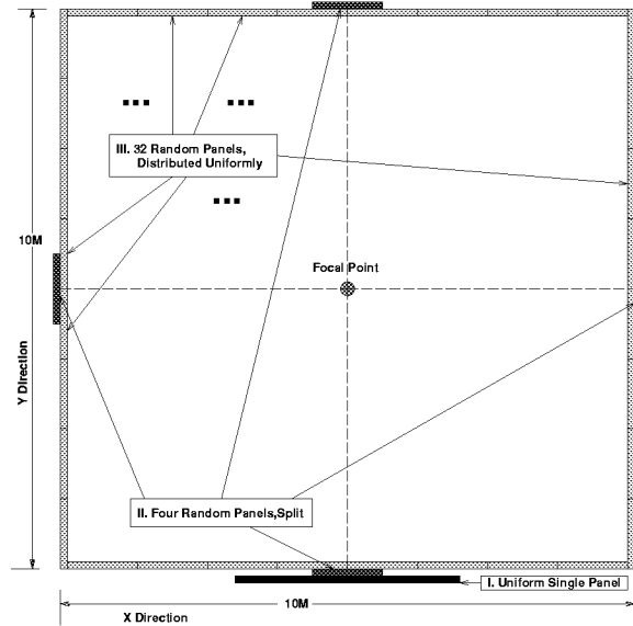
Figure 1: Top View of Room with Three Array Configurations
