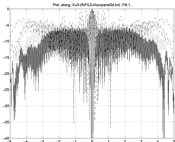
Figure 6: Response for Array II on 10M Line Parallel to X Axis through Aiming point for 500Hz, 1kHz,2kHz and 4kHz
