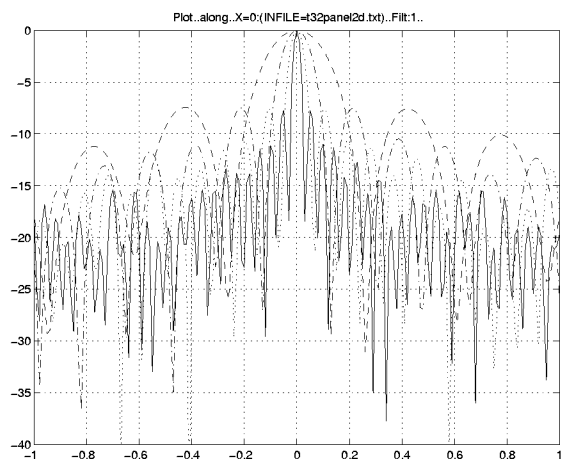
Figure 8: Response for Array III on 2M Line Parallel to X Axis through Aiming point for 500Hz, 1kHz and 4kHz
