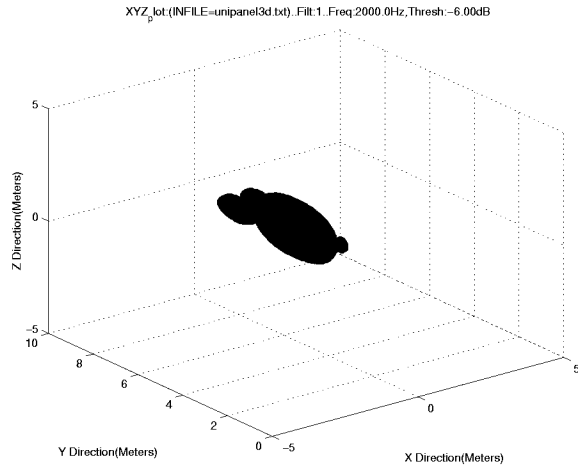
Figure 3: Locus of Points with Response Greater than -6dB at F=2kHz for Array I
