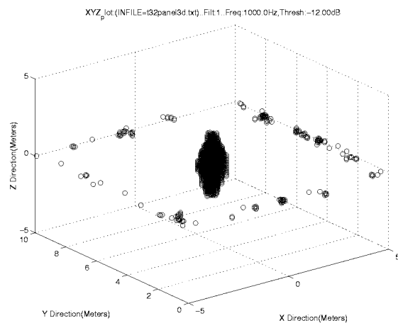
Figure 10: Locus of Points with Response Greater than -12dB at F=1kHz for Array III
