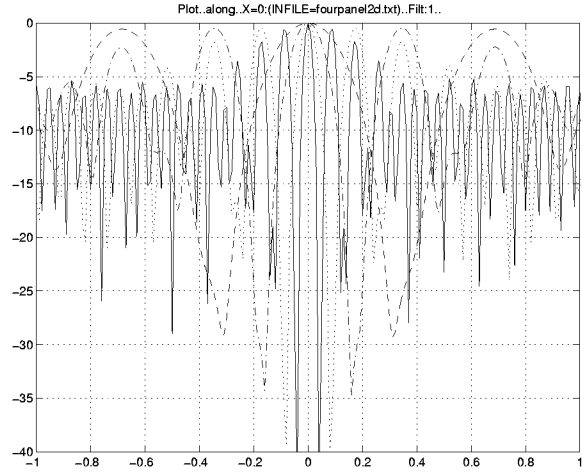
Figure 5: Response for Array II on 2M Line Parallel to X Axis through Aiming point for 500Hz, 1kHz and 4kHz
