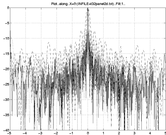
Figure 9: Response for Array III on 10M Line Parallel to X Axis through Aiming point for 500Hz, 1kHz,2kHz and 4kHz
