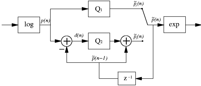
Figure 5: Block diagram of the proposed pitch quantization scheme. A uniform memoryless quantizer, Q_1 is used in parallel with a differential quantizer (the lower branch, including the uniform quantizer Q_2 ).
