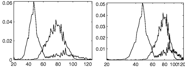
Figure 3: Histogram of pitch periods for female (max value at around 50 samples) and male (max at 80 samples) speakers. Left: linear pitch scale. Right: logarithmic pitch scale.
