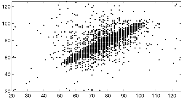
Figure 2: Scatter plot of two consecutive pitch periods for a male speaker.
