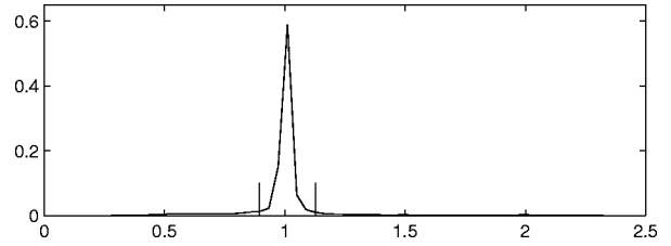
Figure 4: Histogram of the ratio between two consecutive pitch periods. A ratio between 0.9 and 1.11 (the lines) is classified as belonging to the high-correlation group.
