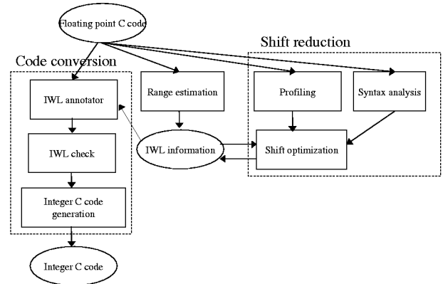
Figure 1. The floating-point to integer C converter design flow.
