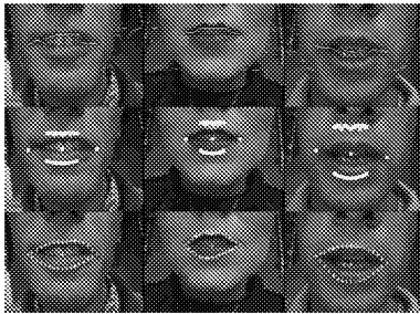
Figure 7: Automatic snake process on open mouth. Top: minima along image. Middle: snake initialization. Bottom: snake results.
