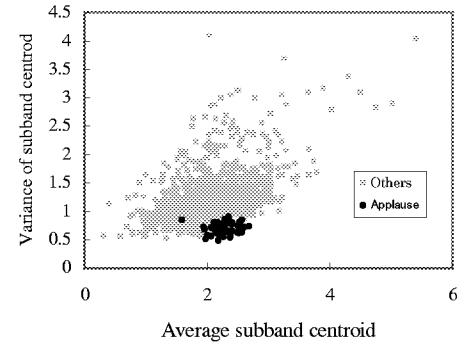
Figure 3. Applause and other sounds in average subband centroid and its variance domain
