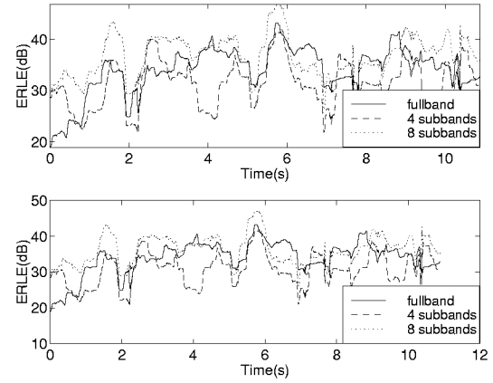
Figure 7: ERLE curves for NLMS in fullband and subband mode for an FIR (top) and IIR QMF bank (bottom), wideband signal
