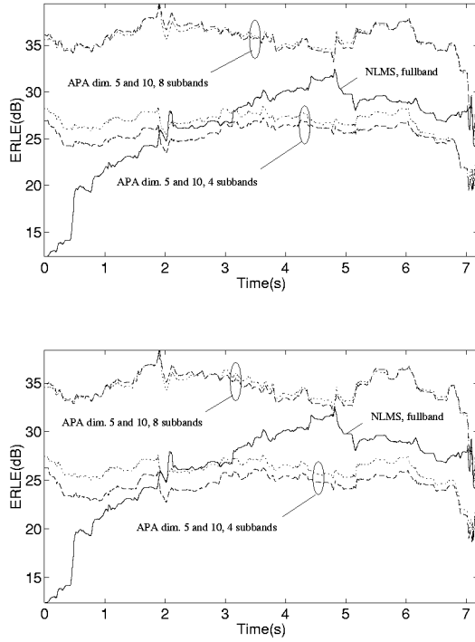
Figure 4: ERLE curves for various order of projection dimensions in fullband and subband mode for an FIR (top) and IIR QMF bank (bottom), narrowband signal
