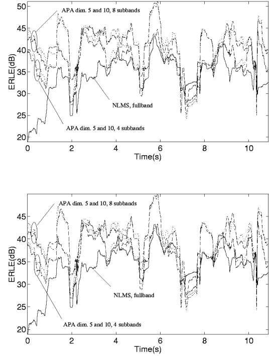
Figure 5: ERLE curves for various order of projection dimensions in fullband and subband mode for an FIR (top) and IIR QMF bank (bottom), wideband signal
