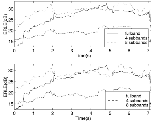
Figure 6: ERLE curves for NLMS in fullband and subband mode for an FIR (top) and IIR QMF bank (bottom), narrowband signal
