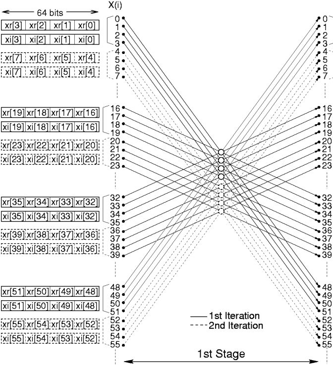
Figure 5: Parallelization of the 1st Stage.
