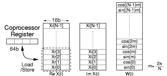
Figure 4: Data Structure for Inputs and Twiddle Factors.
