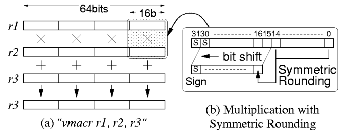
Figure 1: SIMD Multiply-Accumulate Instruction Example.
