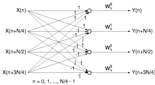
Figure 2: Radix-4 Butterfly Signal Flow.
