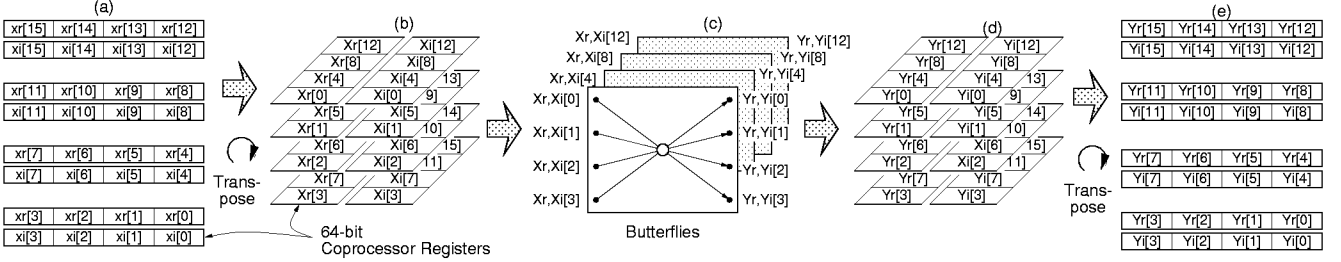
Figure 6: Parallelization of the last Stage.
