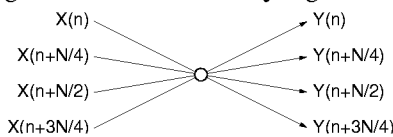
Figure 3: Simplified Radix-4 Butterfly.
