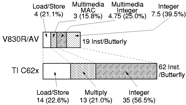
Figure 7: Radix-4 Butterfly Instruction Counts.
