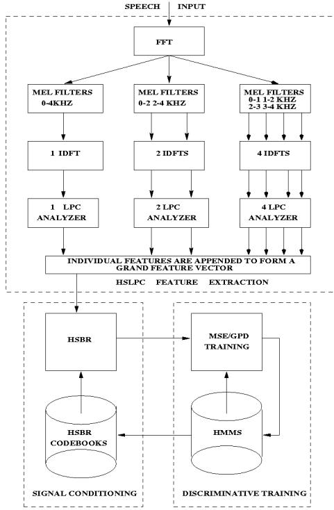
Figure 1. Block diagram of hierarchical subband linear predictive speech analysis with signal conditioned minimum string error rate training.
