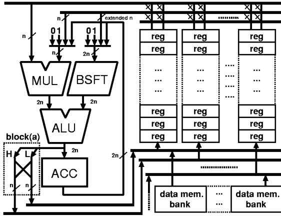
Figure 3: The Structure and Peripherals of MAC unit.
