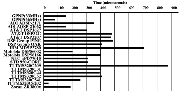
Figure 5: Execution Time for 256-Point FFT[10].
