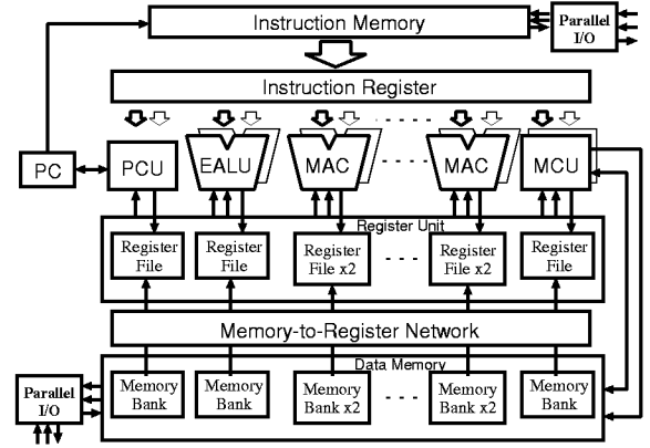
Figure 2: The Organization of the GPNP.
