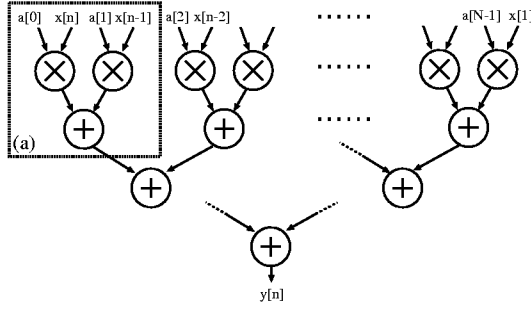
Figure 1: A Signal Flow of FIR Filter.
