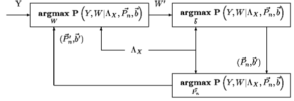
Figure 3: Scheme 2 - for good initial noise guess
