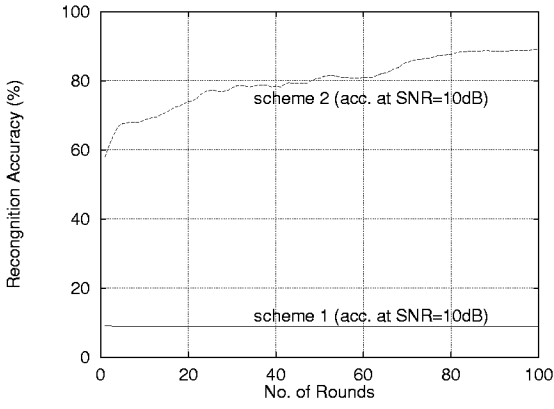
Figure 4: Recognition accuracy of scheme 1 and 2 for the first 100 rounds at SNR=10dB in supervised mode
