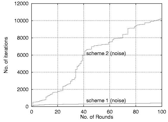
Figure 5: Total number of noise coefficients iterations of scheme 1 and 2 for the first 100 rounds at SNR=10dB in supervised mode
