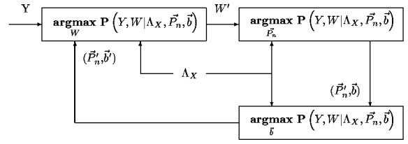
Figure 2: Scheme 1 - for good initial bias guess
