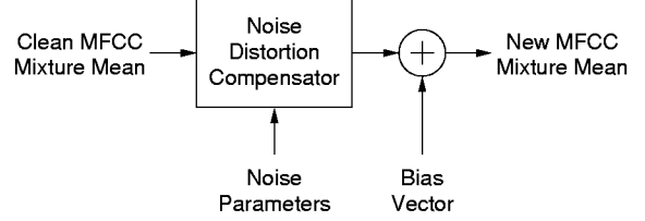
Figure 1: Gaussian mixture mean transformation for ML stochastic matching optimization
