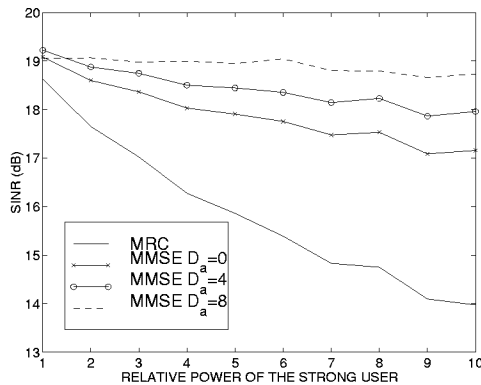
Figure 5: MAI suppression in canonical coordinates with increasing number D_a of auxiliary coordinates.
