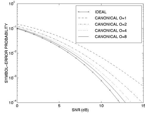
Figure 3: Performance of matched filtering in the ideal (physical) versus canonical coordinates.
