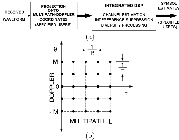
Figure 1: DSP at the receiver in canonical multipath-Doppler coordinates. (a) Overall receiver schematic. (b) The uniformly spaced canonical coordinate grid.
