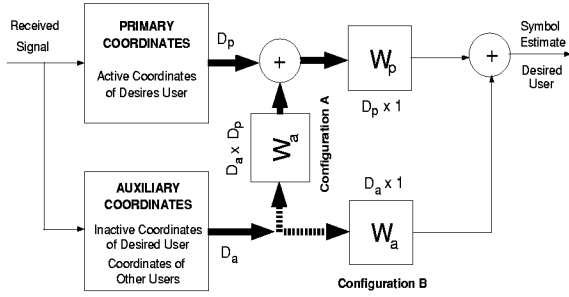
Figure 4: Generic linear receiver structure.
