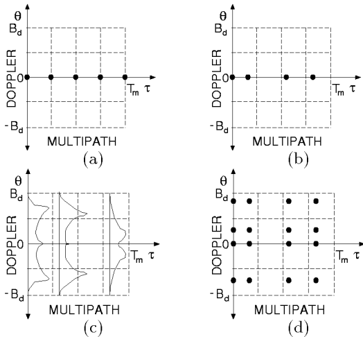
Figure 2: Illustration of various channel models captured by the canonical coordinates via (5). (a) The tapped delay-line multipath model used by the RAKE receiver [2]. (b) Modeling of arbitrary multipath delays. (c) Time-varying extension of (b) via autoregressive modeling of the Doppler spectrum [3]. (d) Time-varying extension of (b) via arbitrary discrete Doppler shifts [4].
