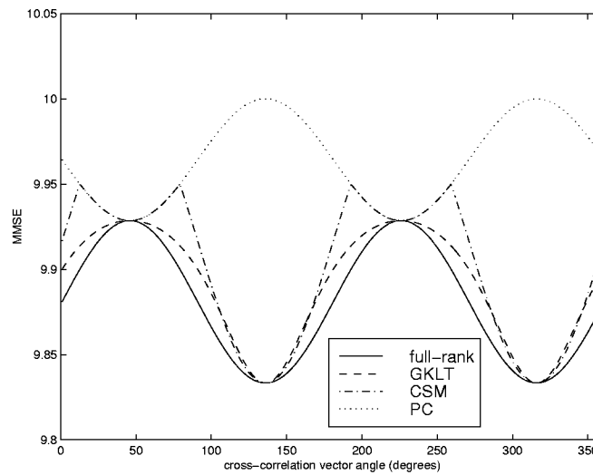
Fig. 3 Relative MMSE performance of the various rank-reduction methods.
