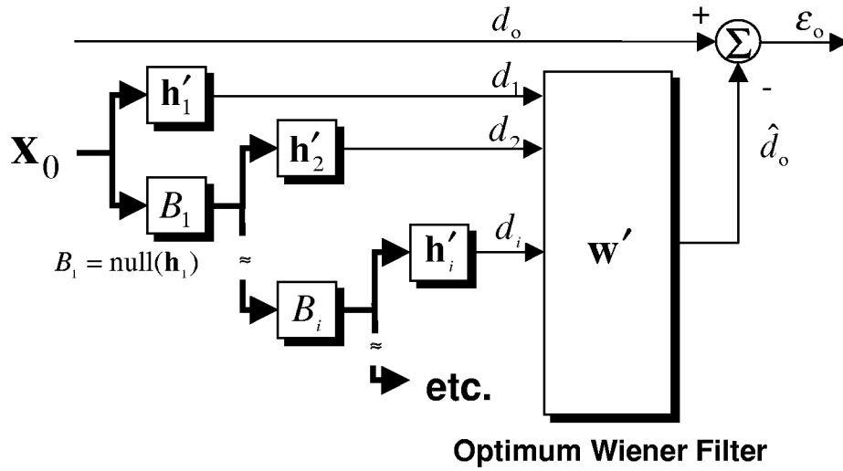
Fig. 2 Multistage Wiener filter structure.
