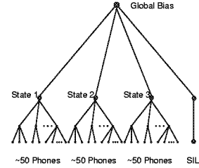
Figure 2: A 150-leaf multiscale tree with richer structure
