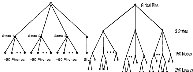
Figure 1: Modeling dependence above the 150 triphone state clusters using multiscale trees with (a) 150 and (b) 250 bias-classes.
