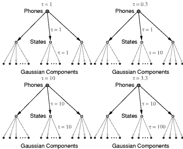
Figure 3: Structured priors used for SMAP adaptation
