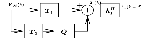
Figure 2: MMSE-ZF Receiver
