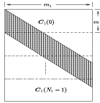
Figure 1: The Code Matrix \mathbf{C}_1
