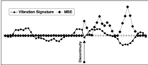
FIGURE 5. Changes in MSE at the Due to "Fault Insertion" from No Defect (B) to Half Gear Tooth Removed (J)
