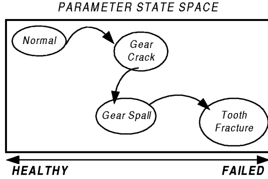
FIGURE 2. Map of Trajectory Through Parameter Space.
