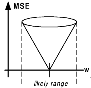
FIGURE 1. Probability Measure Over Single Parameter
