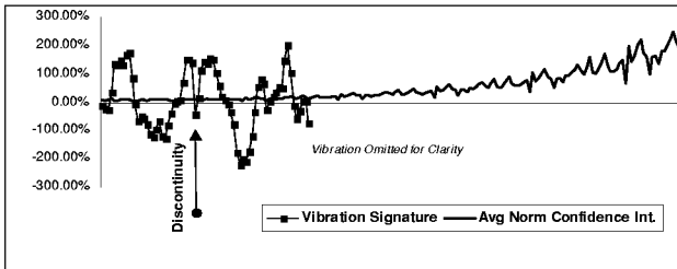
FIGURE 6. Average Changes in (Normalized) Confidence Intervals at the Same Transition
