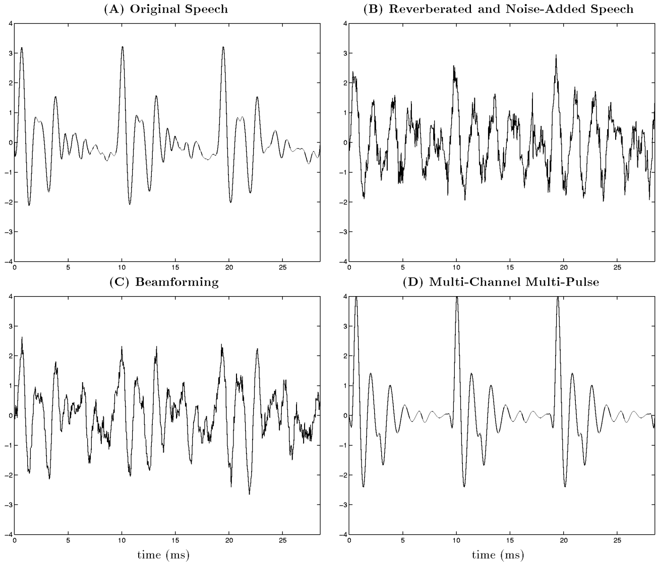
Figure 3. Simulation Results: A reverberated speech segment enhanced via beamforming and the proposed multi-channel multi-pulse LPC method.
