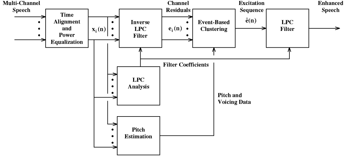
Figure 1. Outline of the Multi-Channel Multi-Pulse (MCMP) Algorithm
