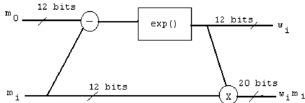
Figure 8: datapath to compute w_i m_i and w_i .
