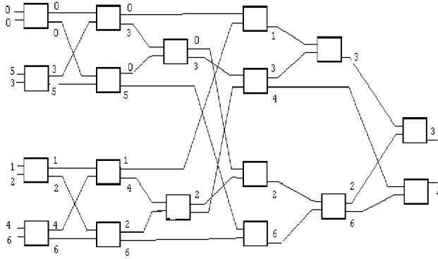
Figure 5: Modified sorting network
