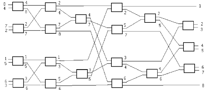
Figure 3: Sorting network for sequence of size eight.
