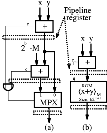
Figure 3: Modular addition with CPLD. (a) MPX-Add and MPX-Add-Pipe. (b) ROM-Pipe.
