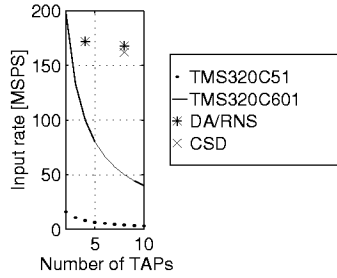
Figure 4: Comparison of programmable DSPs and FPL two channel DWT filter banks.
