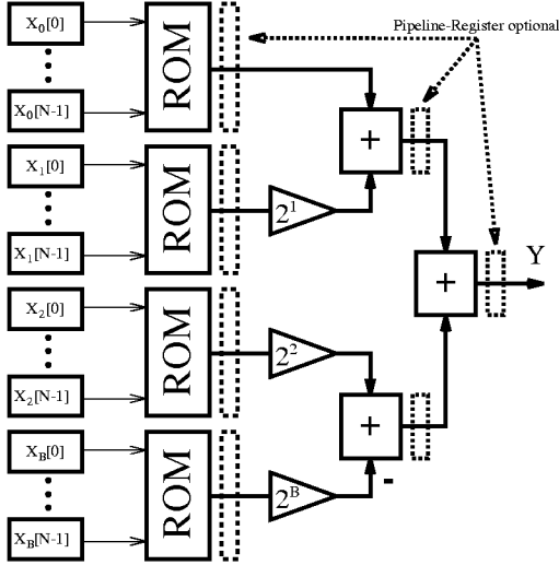
Figure 2: Maximum speed DA implementation.
