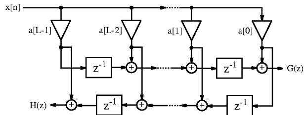
Figure 1: Orthogonal two channel filter bank in transposed FIR form.
