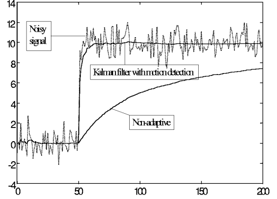
Figure 1- The result of Kalman filtering, using motion detection, in comparison with non-adaptive filtering when SNR is 20dB and \Gamma=3.29 .
