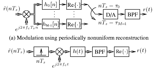
(b) Modulation using uniform reconstruction and a piecewise-constant filter with nonuniformly spaced transitions
