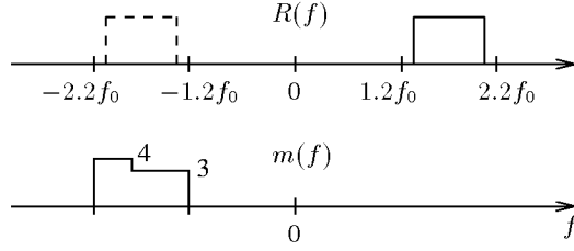
Figure 6: Example bandpass signal spectrum and corresponding function m(f) .
