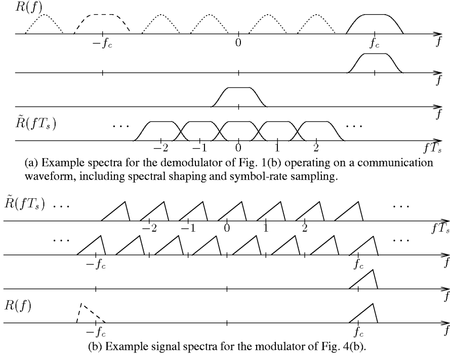
Figure 3: Spectral descriptions of the demodulation and modulation systems.
