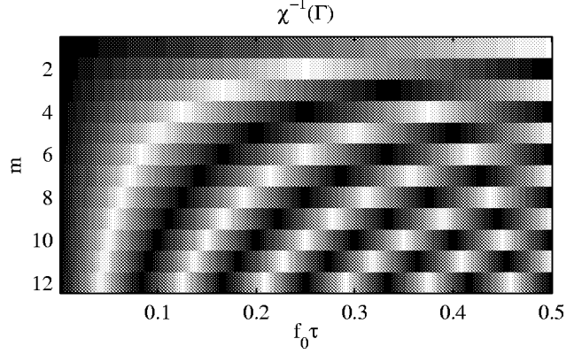
Figure 5: Inverse condition number of the matrix \Gamma vs. sampling offset \tau and index m for the case of second-order sampling. White indicates a value of 1.
