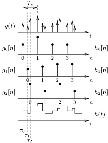
Figure 2: The modulator and demodulator equivalent filters are each related to (discrete-time representations of) their respective polyphase component filters as shown. (In general, modulator and demodulator filters would have different coefficients.)
