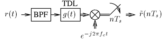
(b) Demodulation using uniform sampling and a TDL with nonuniformly spaced taps.
