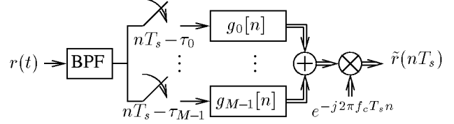
(a) Demodulation using periodically nonuniform sampling.
