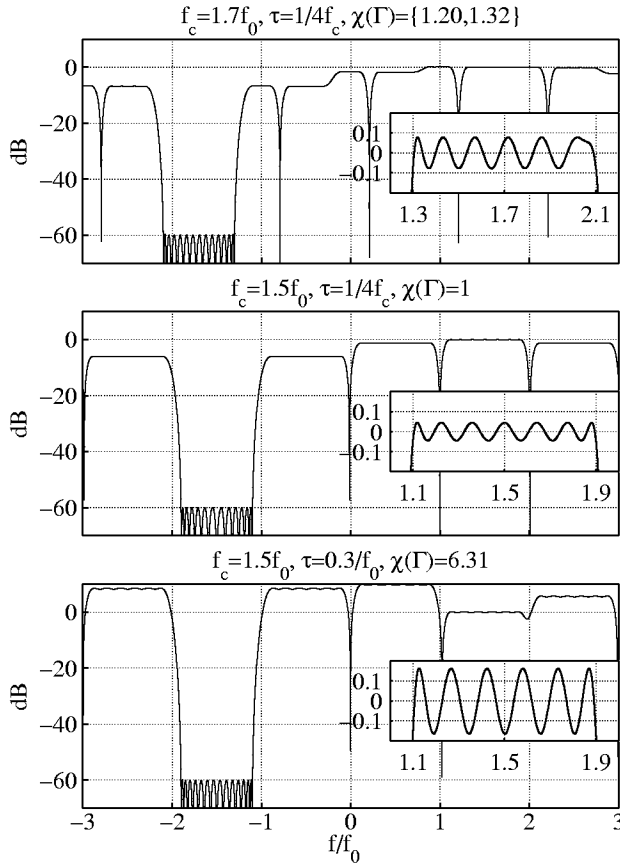
Figure 7: Frequency responses of the example nonuniformly-spaced TDL filters.
