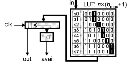
Figure 4: Schematic of encoder PE architecture. A conceptualization of the data storage technique is shown in the LUT.
