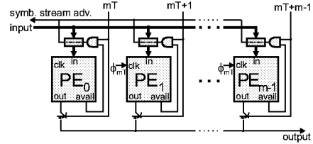
Figure 2: Basic support circuitry for the parallel encoder.
