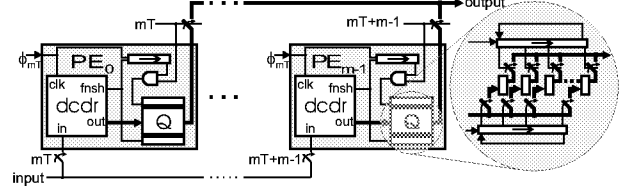
Figure 3: Support circuitry for the parallel decoder. Magnified inset: detail of the queue structure.
