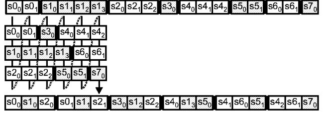
Figure 1: Stream rearrangement: entire codewords are allocated to the (prioritized) first-available PE channels. These are scanned in order bit-by-bit resulting in an output with embedded concurrency.
