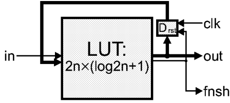
Figure 5: Diagram of the decoder PE architecture. Minimal critical-path delay and overall simplicity of design are evident.
