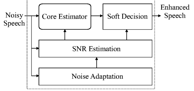
Figure 1: The general structure of the modified MMSE-LSA algorithm.
