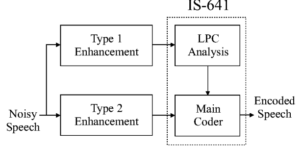
Figure 2: Using two different types of speech enhancement as a pre-processor for the IS-641.
