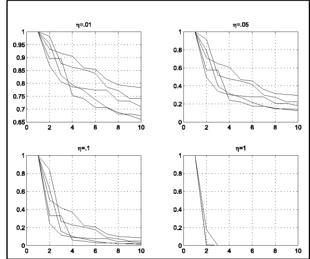
Figure 2: Exponential weighting versus the rank of the word sequence n
