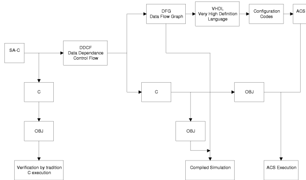
Figure 2. ACS Design Flow Diagram.
