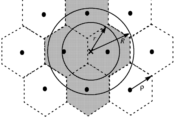
Fig. 2. Lattice structure and search mechanism. Point “x” is the query. A hexagonal lattice structure is shown. r and R are the desired and actual search radius respectively. p is the minimum radius of a sphere that can cover a Voronoi cell.
