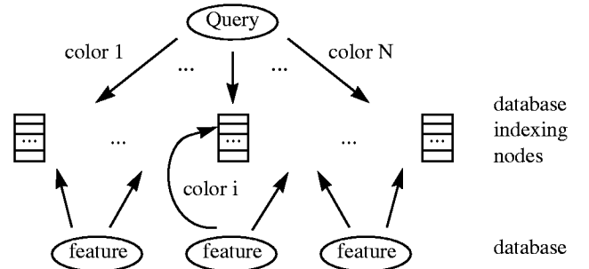
Fig. 1. Basic indexing and search scheme.
