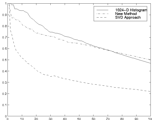
Fig. 3. Precision vs. number of retrievals.
