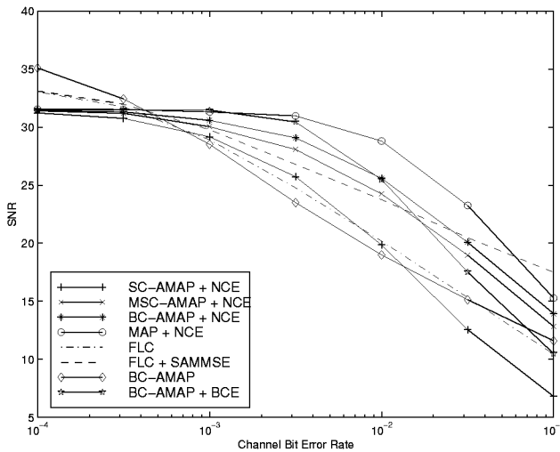
Figure 3: SNR versus channel BER performance of several techniques based on averaging mean-squared error from 10 different channel realizations.
