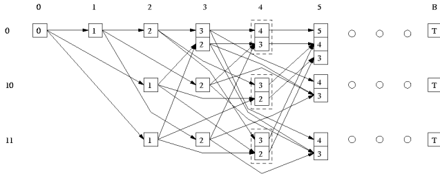
Figure 1: Directed graph representation for VLC decoding/MAP sequence estimation in [6], [7]. The horizontal axis corresponds to bit time and the vertical axis to Huffman-coded symbol choices. The boxes represent decoding states, with the enclosed numbers the length of the symbol sequence required to reach the state.
