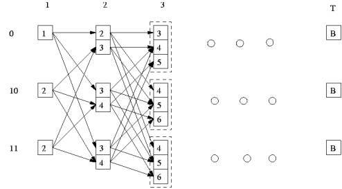
Figure 2: Directed graph representation for VLC decoding/MAP sequence estimation. An approximate method based on this structure was proposed in [1]. The horizontal axis corresponds to symbol time and the vertical axis to Huffman-coded symbol choices. The boxes represent decoding states, with the enclosed numbers the length of the bit sequence required to reach the state.
