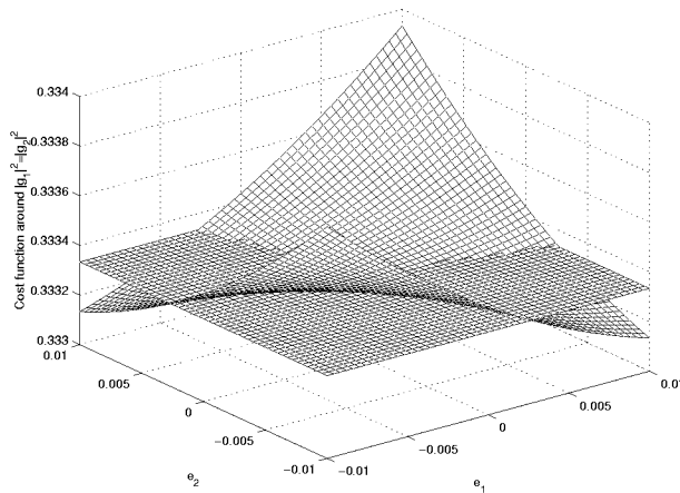
Figure 1. A saddle point ( N = 2 )
