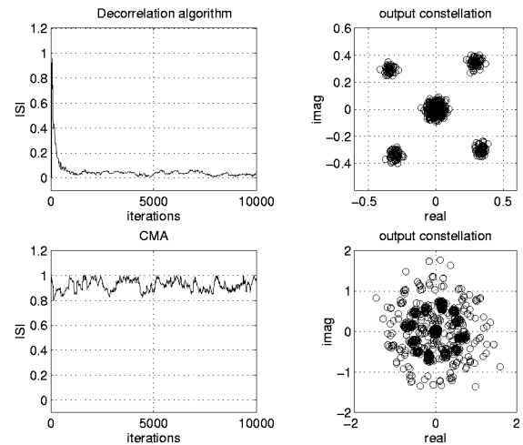
Figure 2. A computer simulation example
