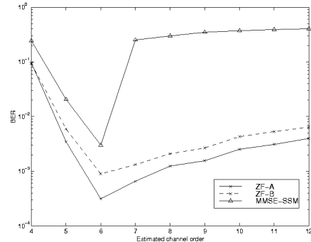
Figure 2. BER vs the estimated channel order. Data length is 350 symbols. SNR=18dB.
