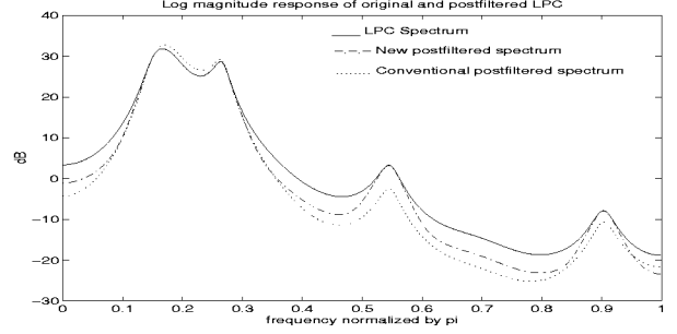
Figure 3: Post-filtered LPC spectra
