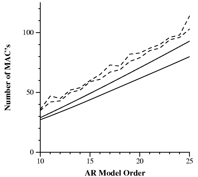
Figure 4: Complexity vs. model order. Solid curves are averages, dashed curves are maximums. For each pair, bottom curve is \beta = 2 , top curve is \beta = 1
