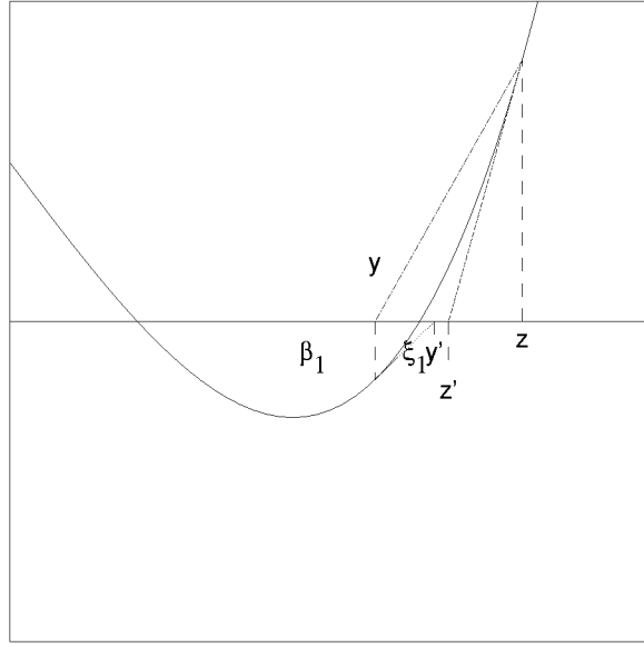
Figure 2: Graphical depiction of the convergence of the second-order Newton iteration
