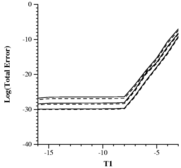
Figure 3: Log LSF error as a function of stopping threshold T_1 . Solid curves are forward deflation, dashed curves are reverse deflation. Predictor orders are (top to bottom): 16, 12, 8.
