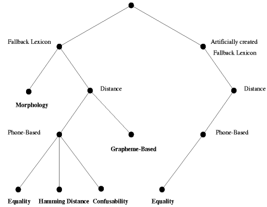
Figure 2: Overview over all HDLA Methods.
