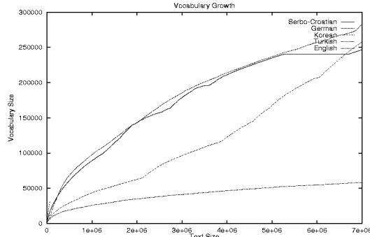
Figure 1: Vocabulary Growth of several Languages.
