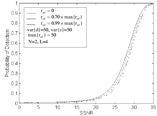
Fig. 4. Maximum error case when d and z are correlated.
