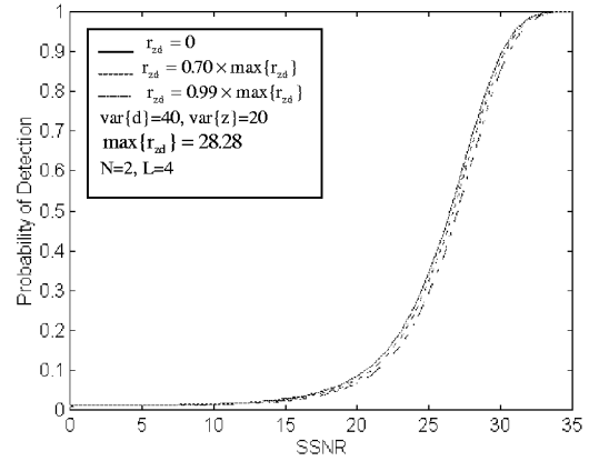
Fig. 3. Typical case when d and z are correlated.
