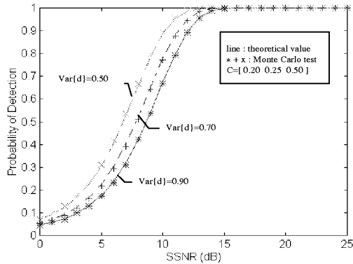
Fig. 1. Probability of detection variation with Var\{d\}
