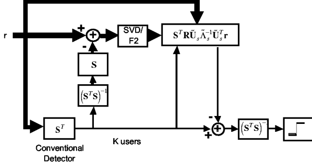
Figure 1: Hybrid semi-blind detector.
