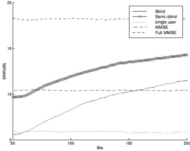
Figure 2: Performance with 7 known and 4 unknown users.
