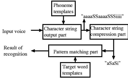
Figure 1: Block diagram of our speaker-independent word recognition algorithm.
