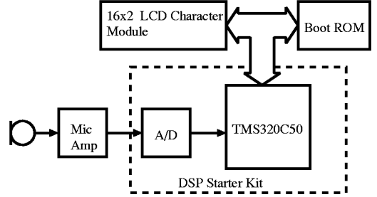
Figure 3: The structure of the processor implementation.
