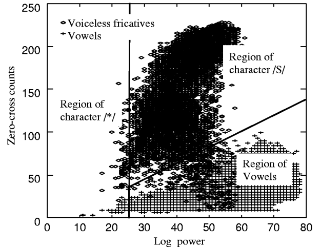
Figure 2: Distribution of voiceless fricatives and vowels in the (frame power, zero-cross counts) plane, and the discriminant diagram for classifying pause, voiceless fricatives and vowels
