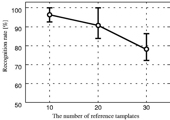
Figure 4: The range of the recognition rate relative to the number of reference templates, with the average indicated by a circle.
