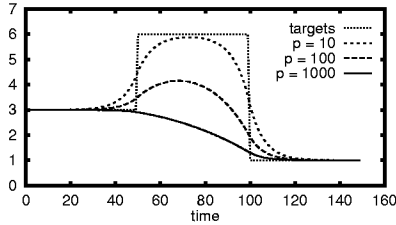
Figure 5: Hidden dynamic trajectories with time constants of 10, 100 and 1000 units for the centre segment.
