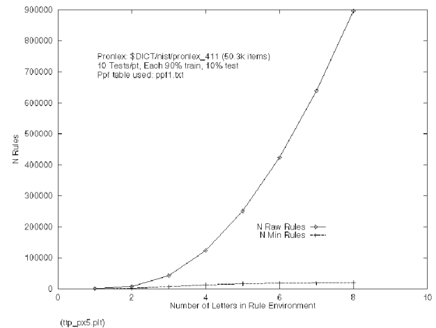
Fig. 4. Effect of Deleting Redundant Rules.
