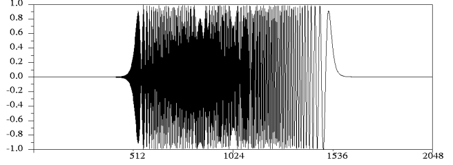
Figure 1: Example of time-stretched pulse p(n) , obtained as inverse DFT of the sequence P(k) in equation (1). Here N=2048 , m=1024 (the sequence has been circularly shifted to center the pulse).
