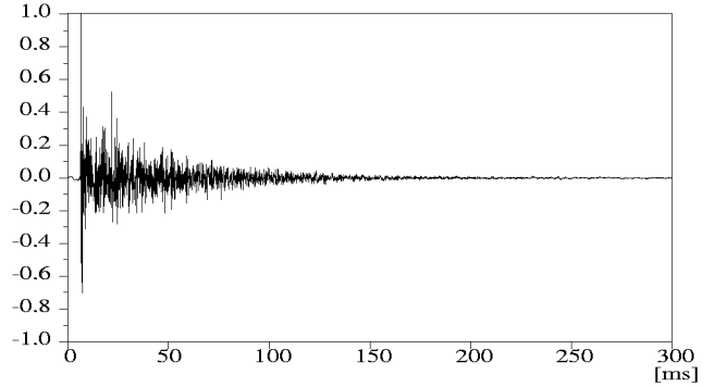
Figure 2: Example of loudspeaker-to-microphone impulse response measured in the experimental room.
