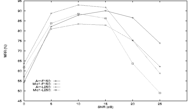
Figure 3: Recognition performance obtained with different model sets corresponding to training sets characterized by different SNRs.
