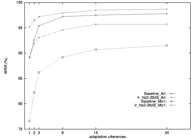
Figure 4: Adaptation results with different amount of speech data for speakers in position F150 , using a single microphone or the microphone array as input. Initial models are either baseline models (curves denoted with Baseline_Mic1 and Baseline_Arr ) or models trained under Ir_Ns2-20dB condition (curves Ir_Ns2-20dB_Mic1 and Ir_Ns2-20dB_Arr ).
