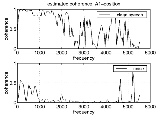
Figure 1: estimated coherence, A1-position
