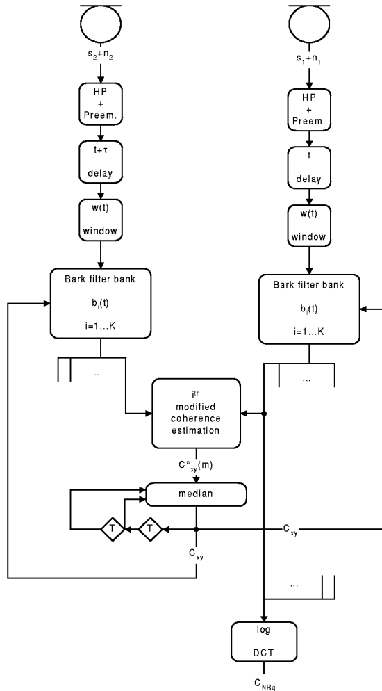
Figure 3: Implemented MFCC-2 system
