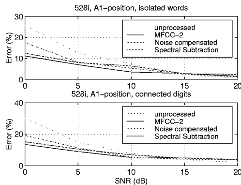
Figure 6: comparison overall performance
