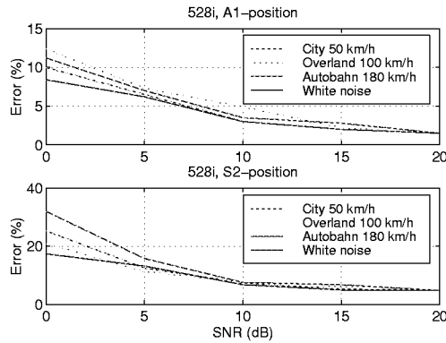
Figure 5: recognition reliability for different mic-positions
