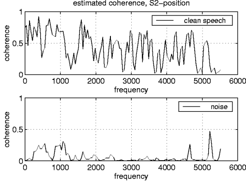
Figure 2: estimated coherence, S2-position
