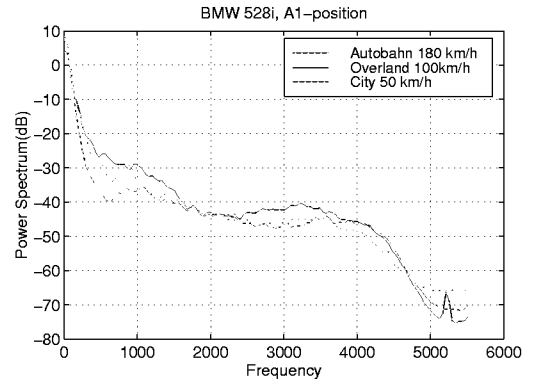
Figure 4: PSD of vehicle noise
