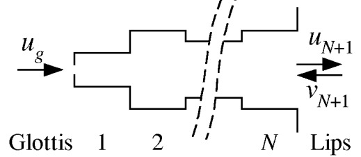
Figure 1. Lossless tube model of the vocal tract
